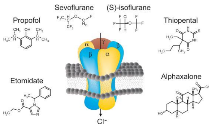
Figure 5: GABA receptor
